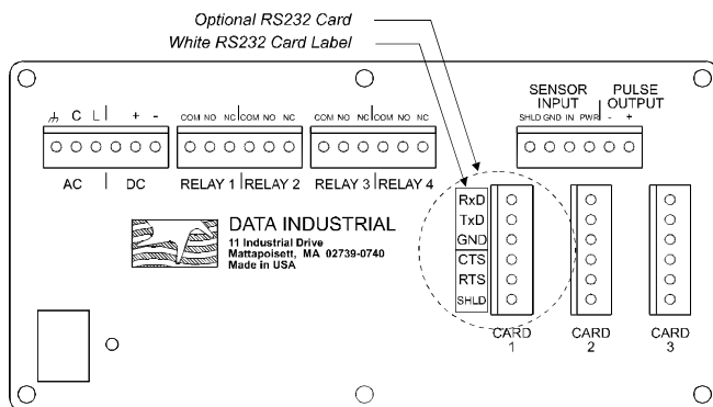
Note: One RS232 Card may be installed per unit. All Option Cards may be installed in any slot configuration.
