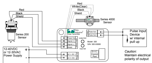
Figure 4: Model 320 Wiring to a generic pulse device and Series 200 or Series 4000
