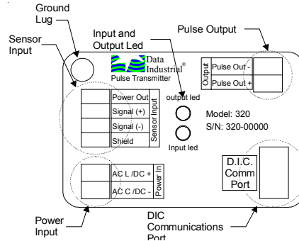
Figure 3: Model 320 Terminal Locations
