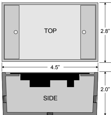
Figure 2: 320 Optional Enclosure Dimensions
