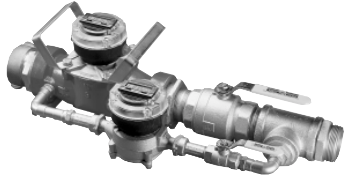
PLMT shown with optional electronic Resettable Registration.
