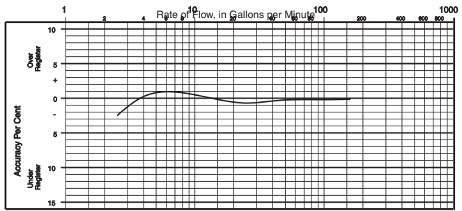
ACCURACY CHART
