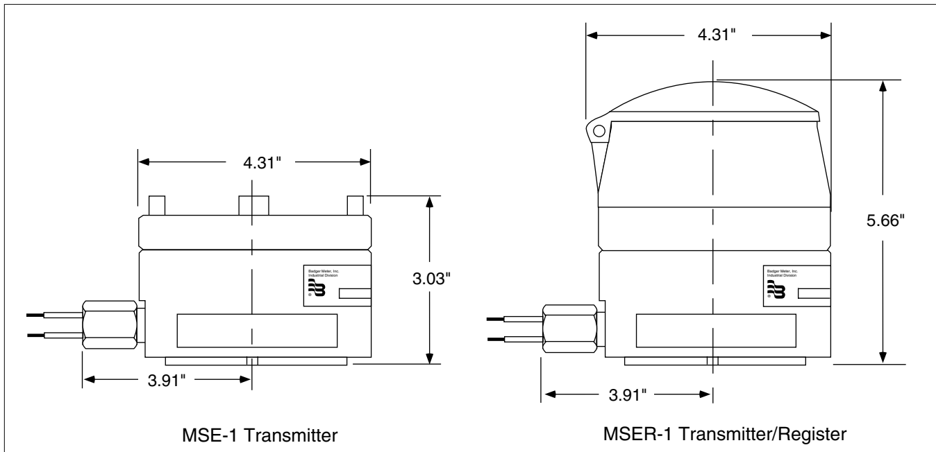
Dimensional Drawings
