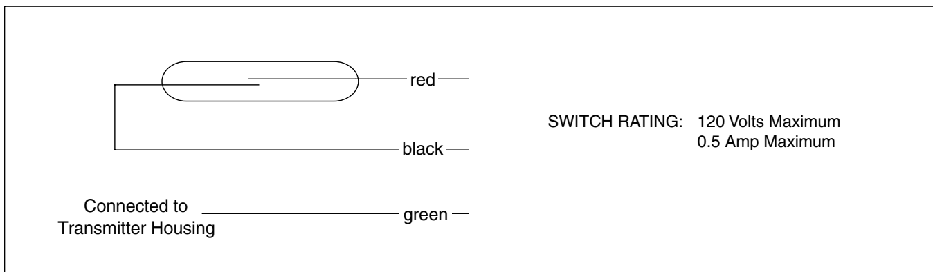
MS-E1 & MS-ER1 Transmitter Wiring Diagram
