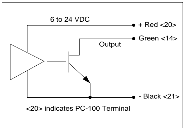
Magnetoresistive Sensor
