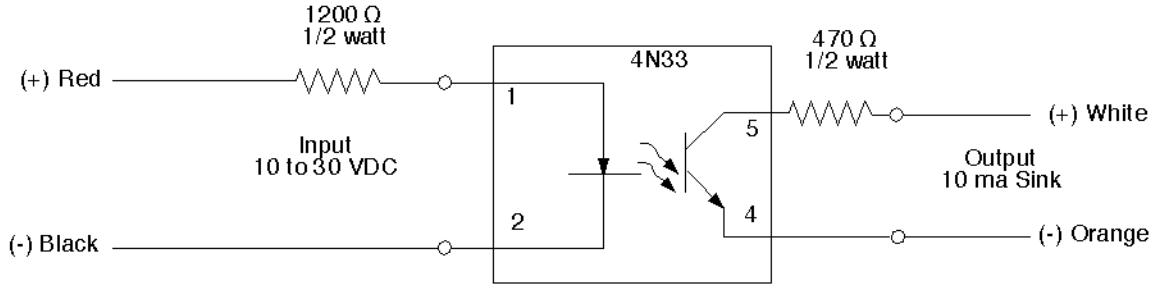
EQUIVALENT CIRCUIT
