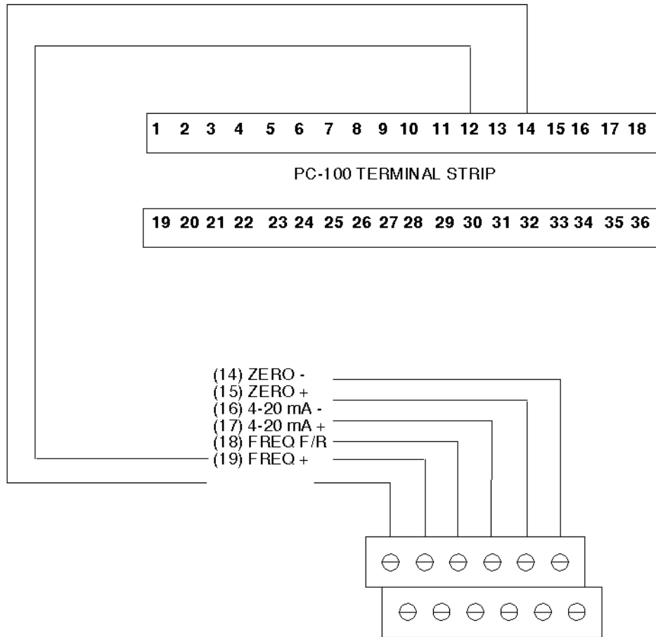
Terminal Strip on Micro Motion Transmitter
