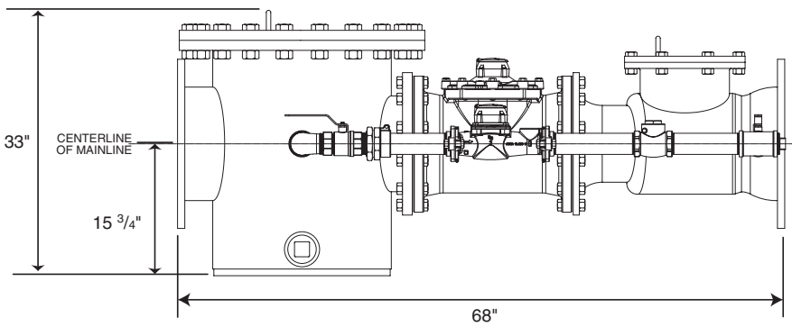
Illustration includes optional 2nd shutoff valve on bypass.
